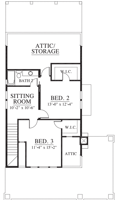
SECOND FLOOR PLAN (668 HEATED SQ. FT.)
