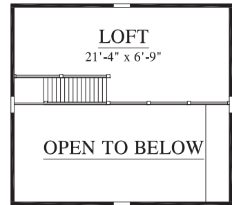
LOFT FLOOR PLAN (195 HEATED SQ. FT.)
