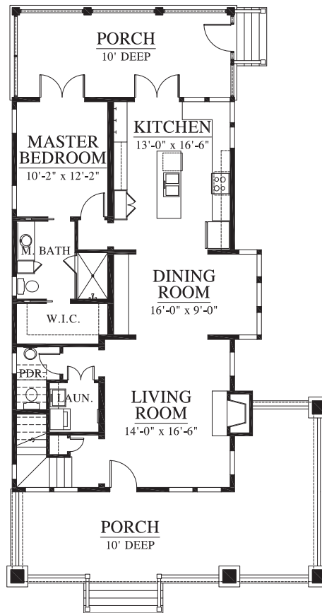
FIRST FLOOR PLAN (1,133 HEATED SQ. FT.)
