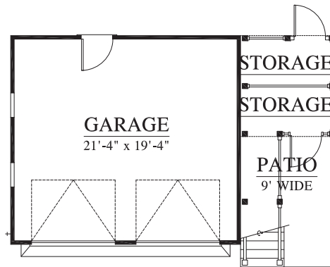
FIRST FLOOR PLAN (440 UNHEATED SQ. FT.)
