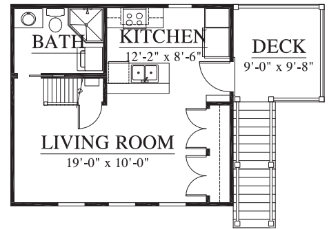
SECOND FLOOR PLAN (440 HEATED SQ. FT.)
