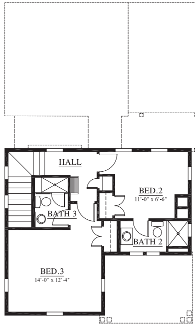
THIRD FLOOR PLAN (528 HEATED SQ. FT.) TOWER FLOOR PLAN (110 HEATED SQ. FT.)
