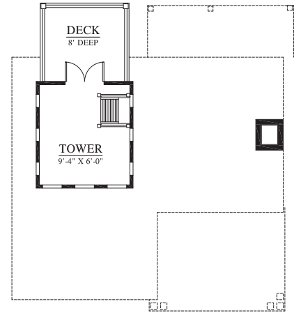
THIRD FLOOR PLAN (528 HEATED SQ. FT.) TOWER FLOOR PLAN (110 HEATED SQ. FT.)
