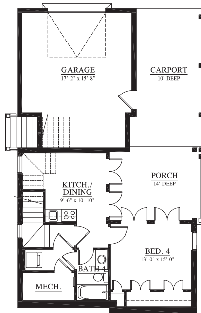
FIRST FLOOR PLAN (520 HEATED SQ. FT.) SECOND FLOOR PLAN (925 HEATED SQ. FT.)
