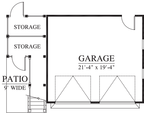
FIRST FLOOR PLAN (440 UNHEATED SQ. FT.)
