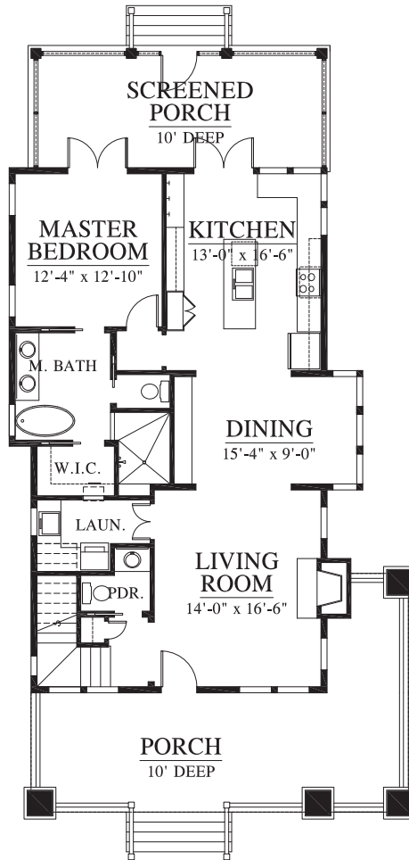
FIRST FLOOR PLAN (1,175 HEATED SQ. FT.)
