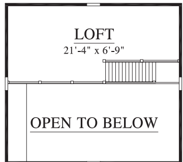
LOFT FLOOR PLAN (195 HEATED SQ. FT.)
